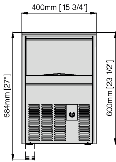
Vue frontale Front view
